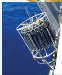
© Digna Ruveda CTD sensor equipped with water sampling rosette deployed at the BATS station.
